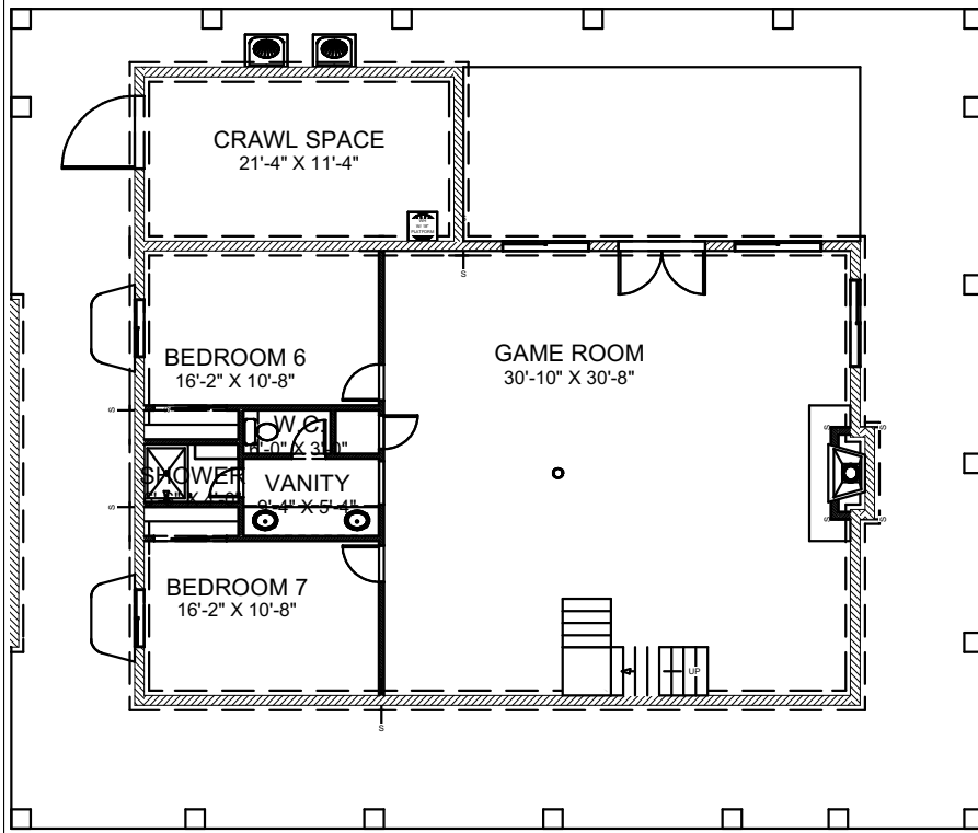
BASEMENT
